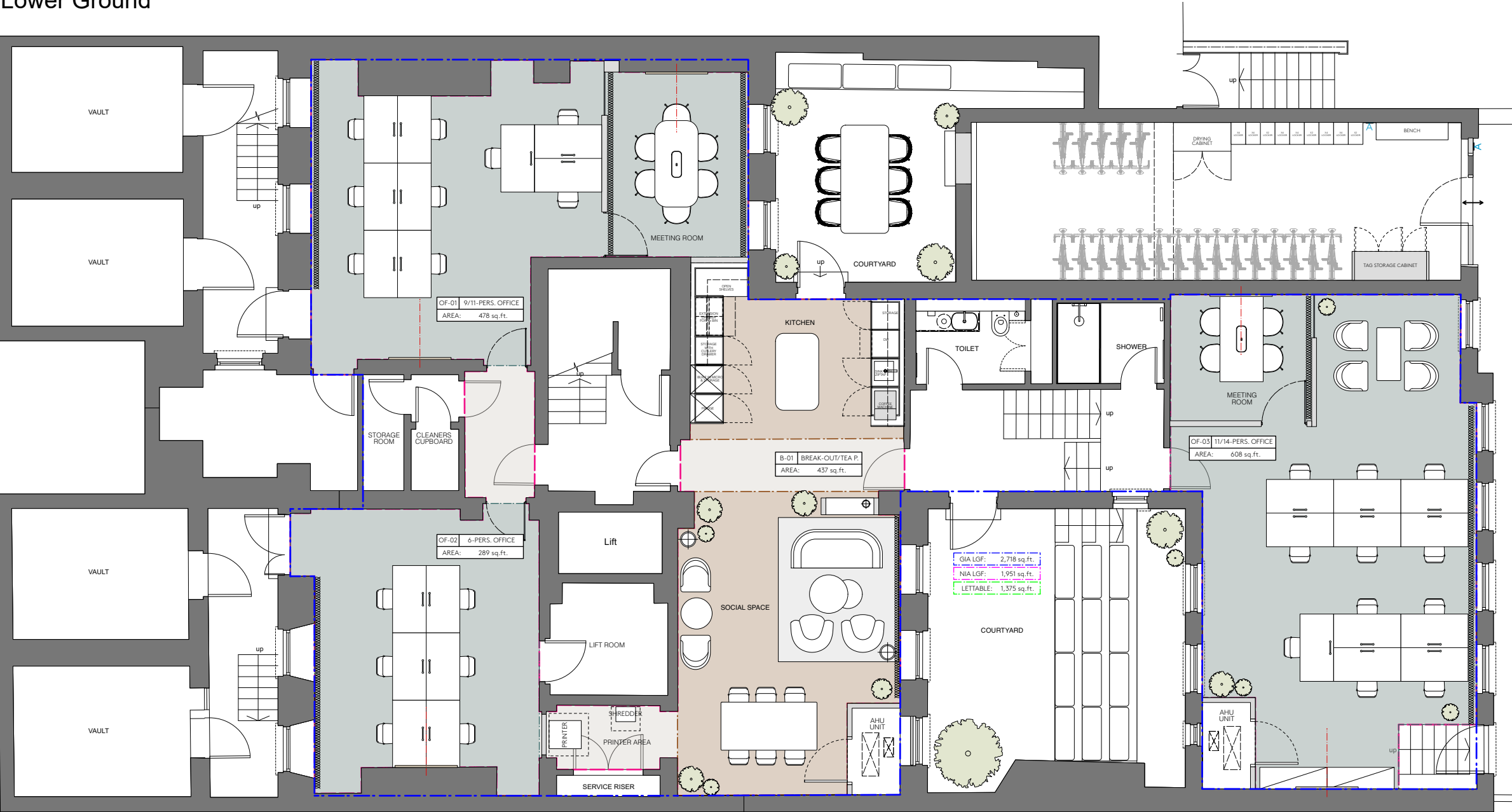
1 GA PLAN - LOWER GROUND FLOOR Scale: 1:50
