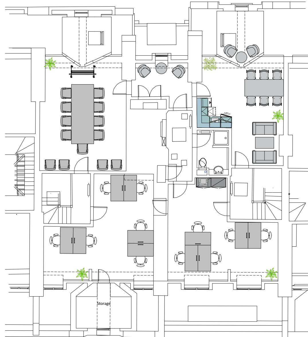
Proposed Fourth Floor Plan
